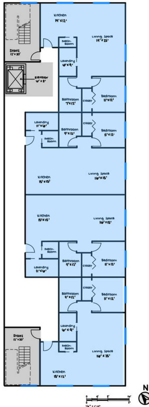
ONE-BEDROOM APARTMENTS FLOOR PLAN
