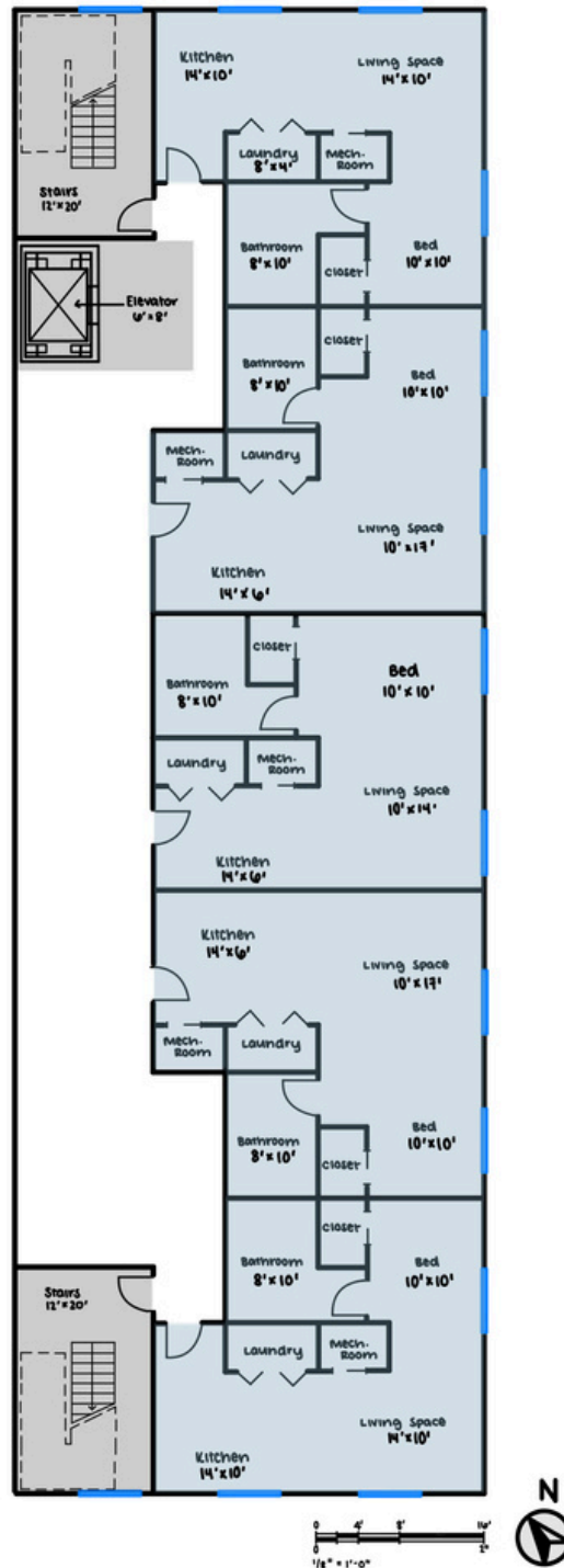
STUDIO APARTMENTS FLOOR PLAN
