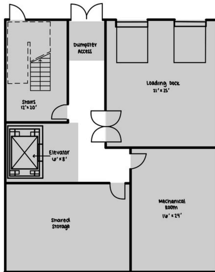
SUB BASEMENT FLOOR PLAN
