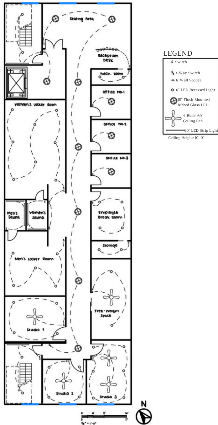
PILATES REFLECTED CEILING PLAN
